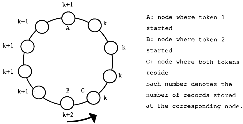
Fig. 3.3.3. The maximum number of records stored at a node with protocol T-2.
